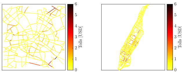
Fig. 7. Optimal road tolls in USD for Berlin (left) and NYC (right).
