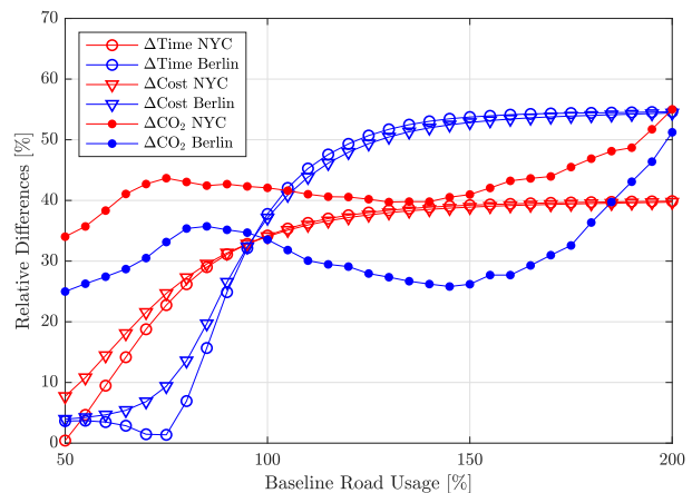
Fig. 9. Relative difference in travel time, cost, and emissions, between AMoD and I-AMoD in Berlin and in NYC.
