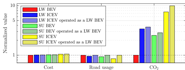
Fig. 8. The optimal solution for different vehicles' configurations for NYC with a 100% baseline road usage shows the impact of the vehicle category and the powertrain type on the optimal system performance and operation.
