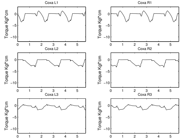
Fig. 7. Coxa torques during walking (on the x -axis time in seconds is shown).
