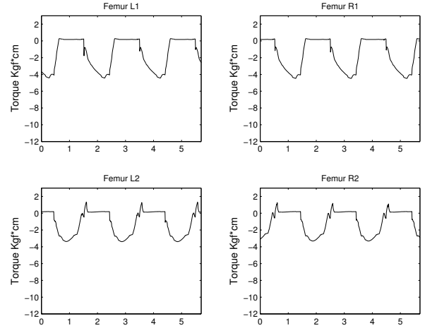
Fig. 8. Femur torques during walking (on the x -axis time in seconds is shown).
