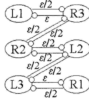
Fig. 6. CPG neuron connections.
