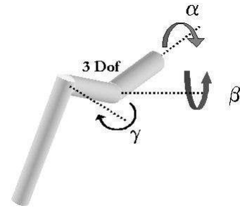
Fig. 2. Middle leg structure (not in scale).
