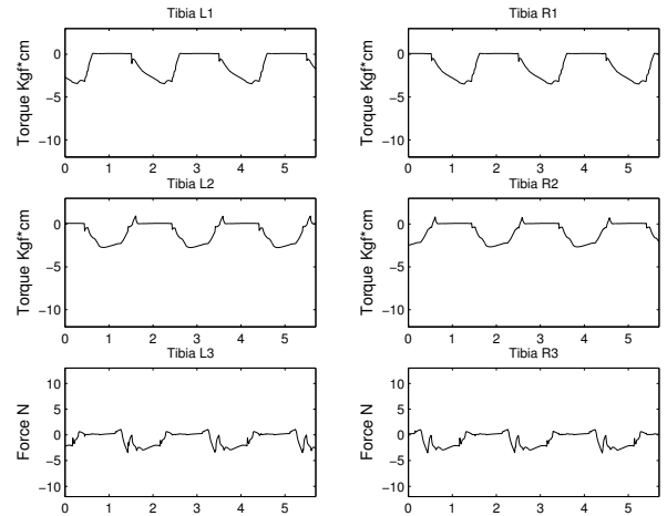
Fig. 9. Tibia torques and forces during walking (on the x -axis time in seconds is shown).
