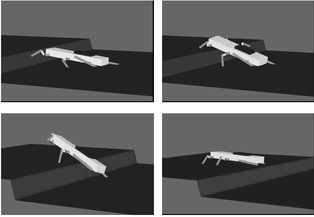
Fig. 10. Climbing a 6 cm (150 % of robot CoM height) obstacle.
